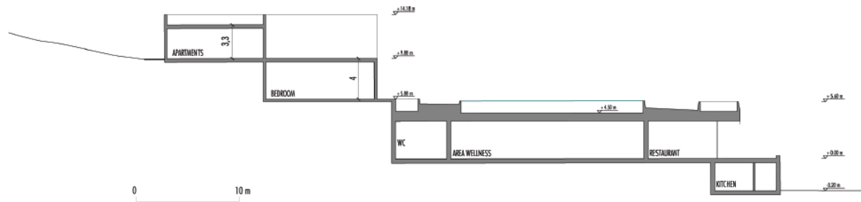
D-D' SECTION
