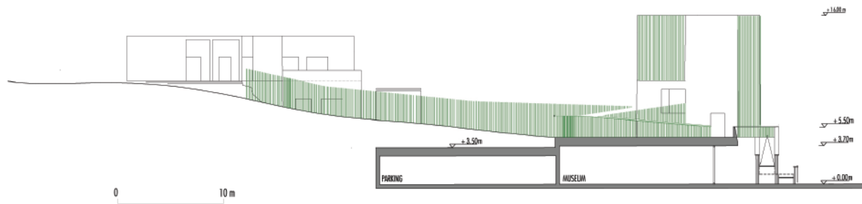
C-C' SECTION
